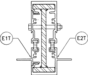
MULLION 'M1'
