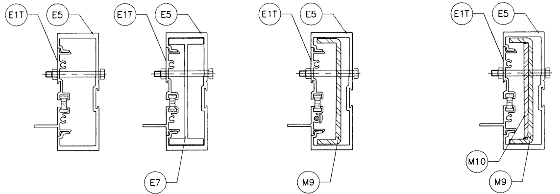
MULLION 'MD1'
