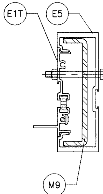
MULLION 'MD3'
