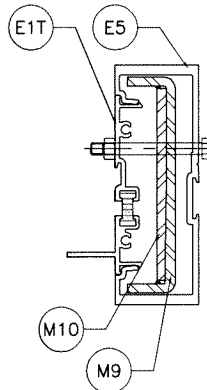
MULLION 'MD4'
